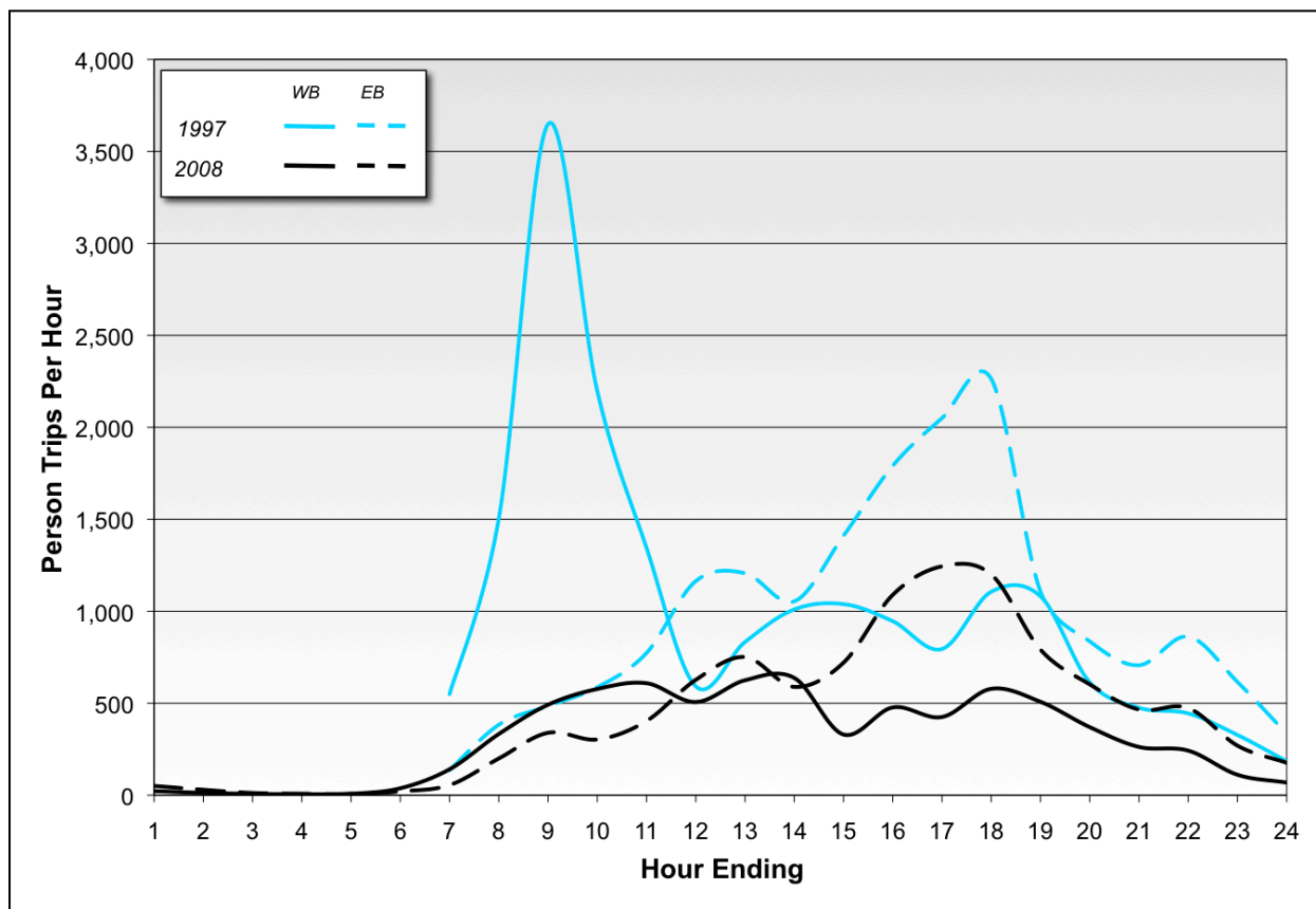
Figure 3.6 – Carpool/Vanpool Trip Patterns Across UBC/UEL Screenline, 2008 vs. 1997
