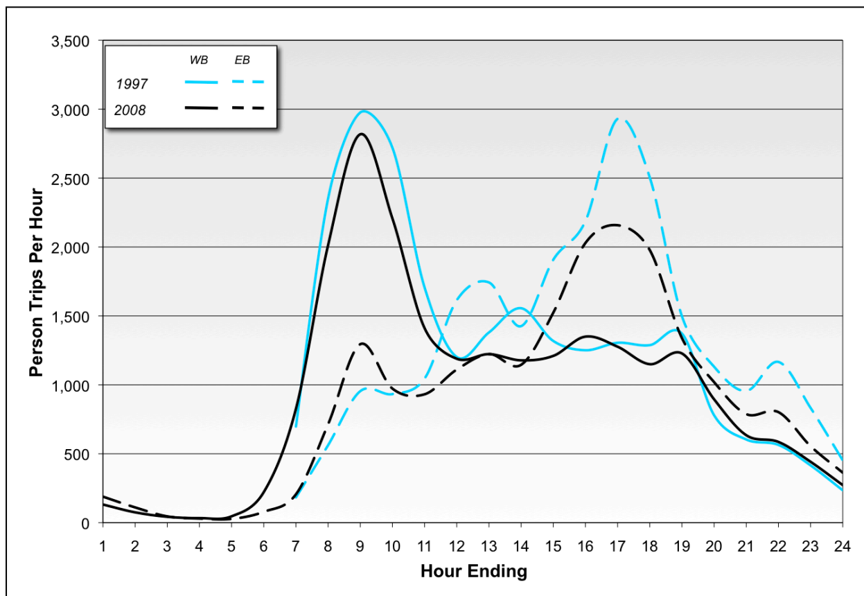
Figure 3.4 – SOV Trip Patterns Across UBC/UEL Screenline, 2008 vs. 1997
