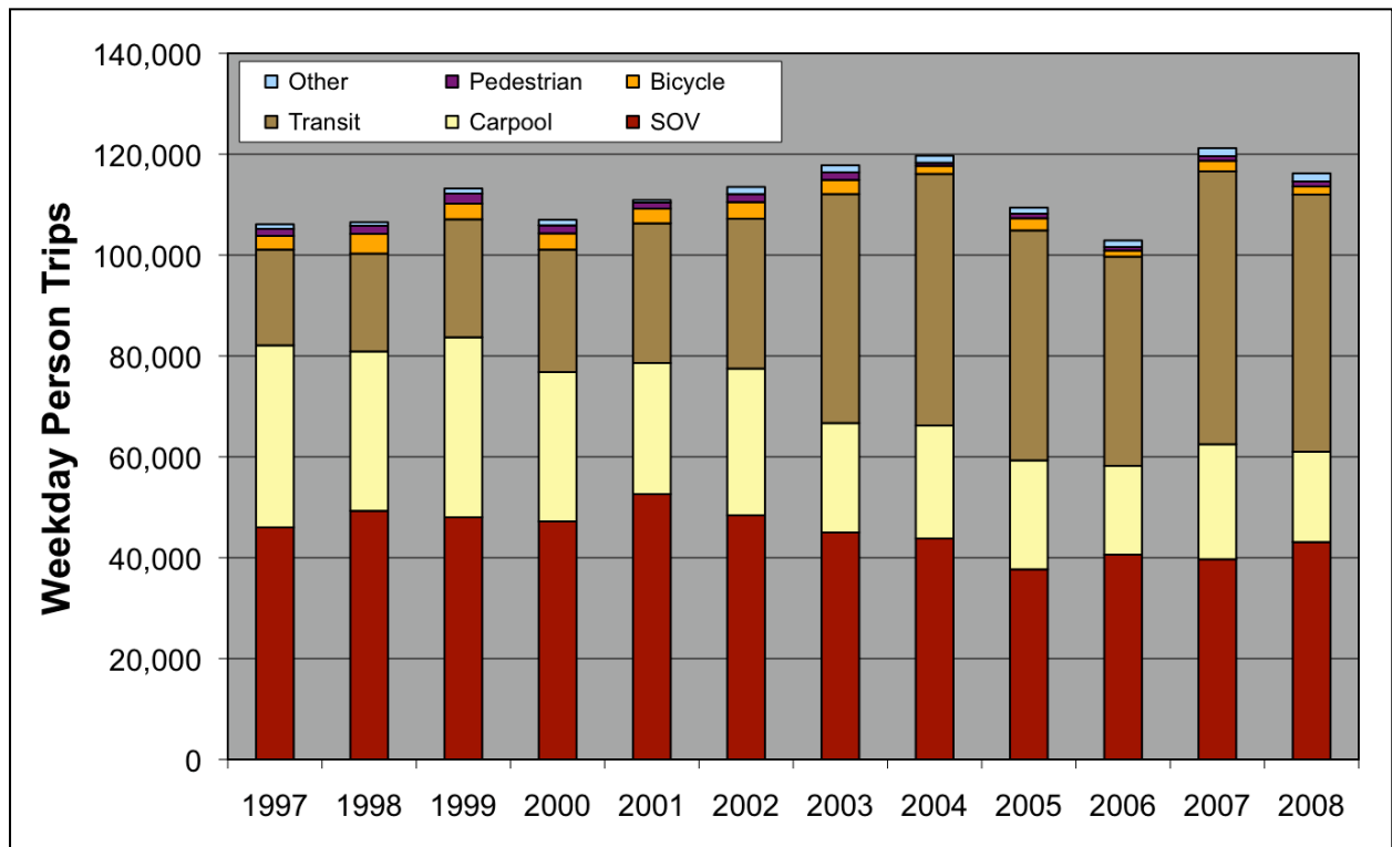
Figure 2.1 – Weekday Person Trips Across UBC/UEL Screenline, 1997–2008
