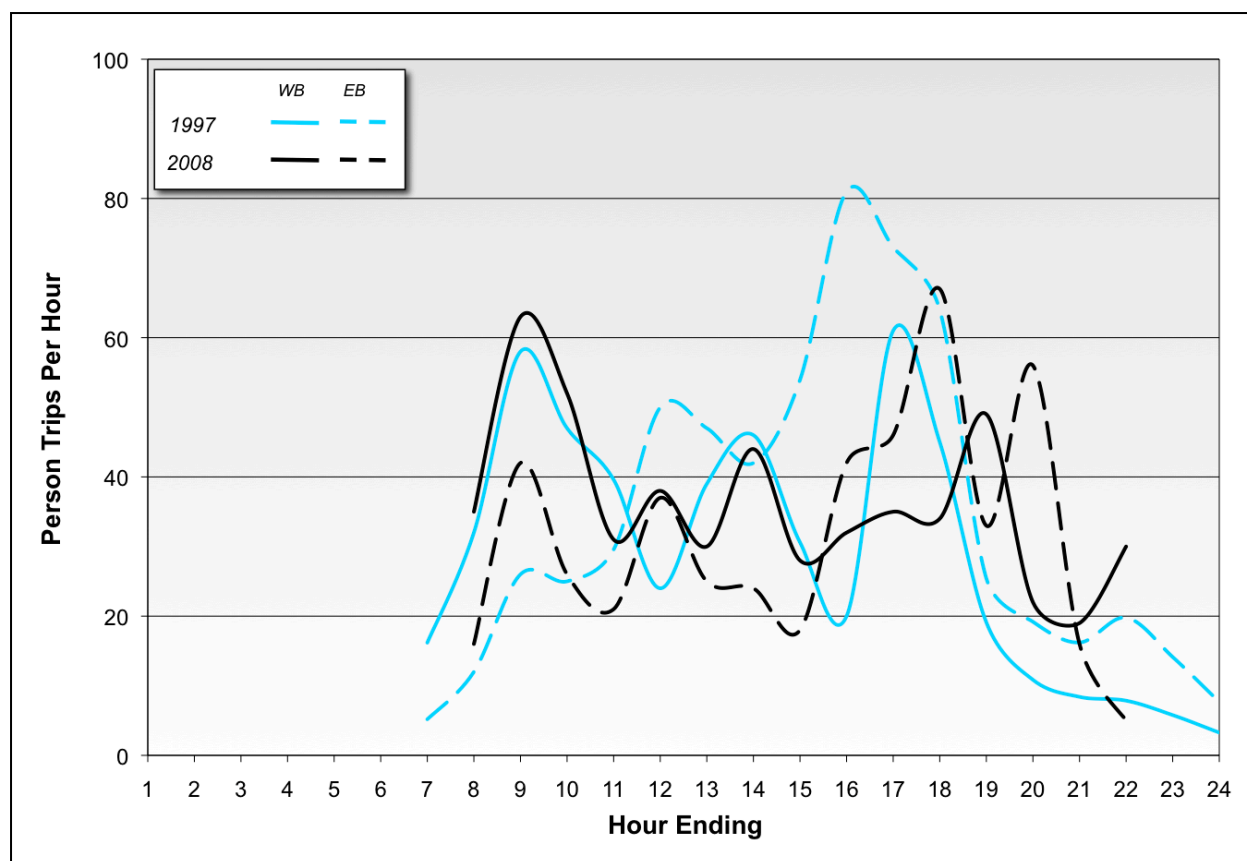
Figure 3.10 – Pedestrian Trip Patterns Across UBC/UEL Screenline, 2008 vs. 1997
