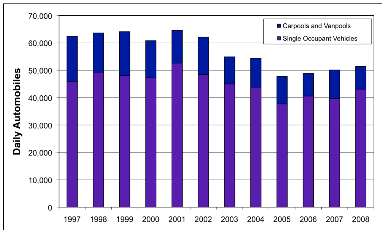
Figure 3.7 – Weekday Automobile Volumes Across UBC/UEL Screenline, 1997–2008
